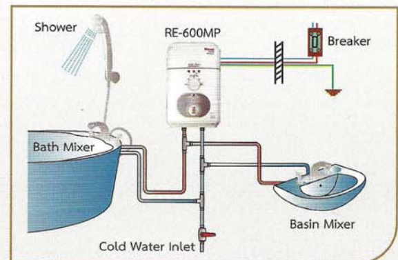
Double Pipe Installation
