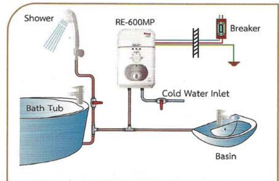
Single Pipe Installation
